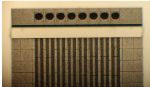
Figure 3: OptoCplrLT™ after HAST demonstrating good structural integrity
